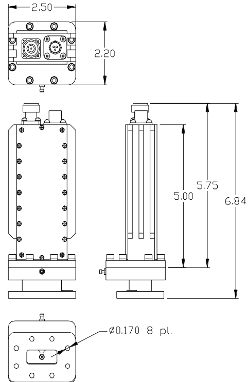
LNA with optional Input Isolator
